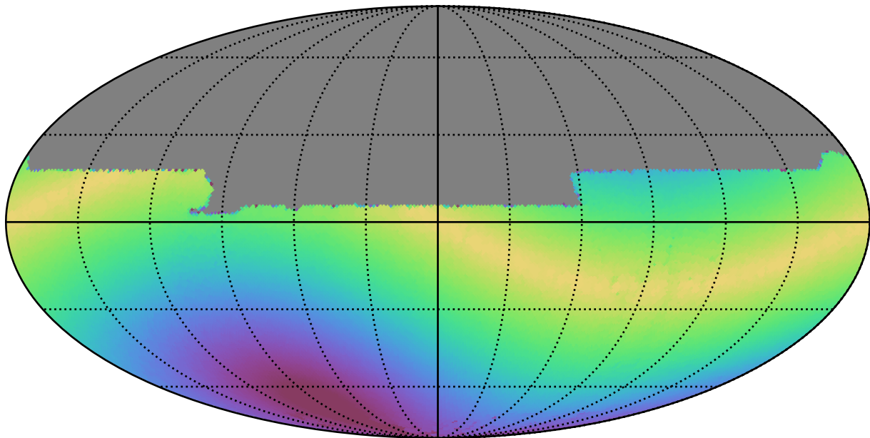
early_u_fpextra3.0_v3.4_10yrs All sky y band: Max solarElong
