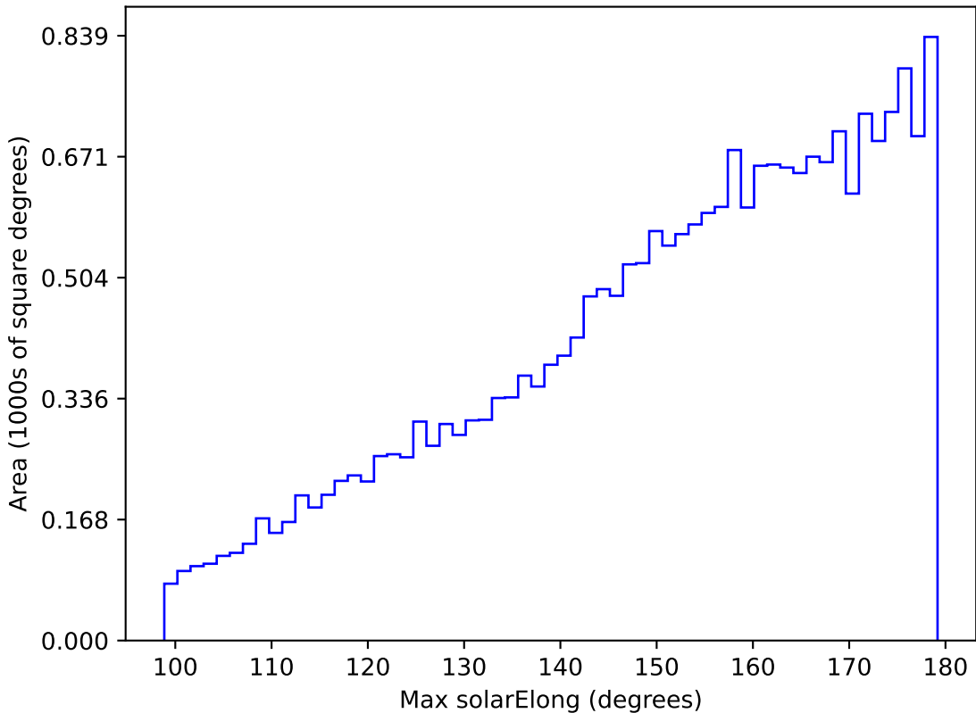
early_u_fpextra3.0_v3.4_10yrs All sky y band: Max solarElong
