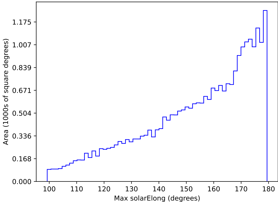
early_u_fpextra3.0_v3.4_10yrs All sky r band: Max solarElong
