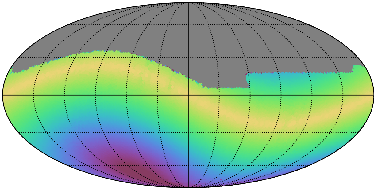
early_u_fpextra3.0_v3.4_10yrs All sky i band: Max solarElong
