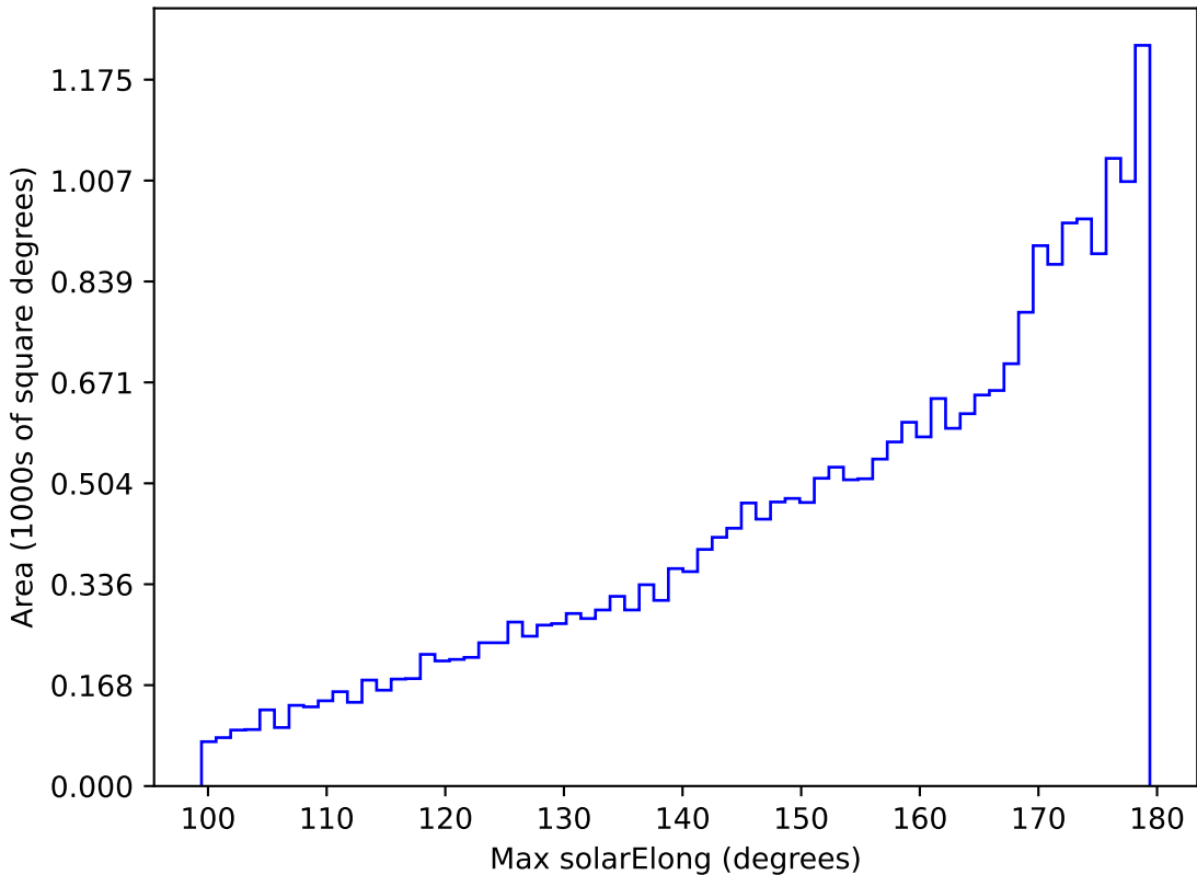
early_u_fpextra3.0_v3.4_10yrs All sky i band: Max solarElong
