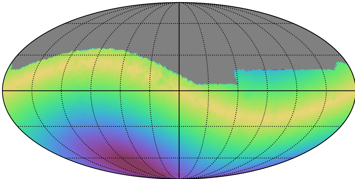
early_u_fpextra3.0_v3.4_10yrs All sky g band: Max solarElong
