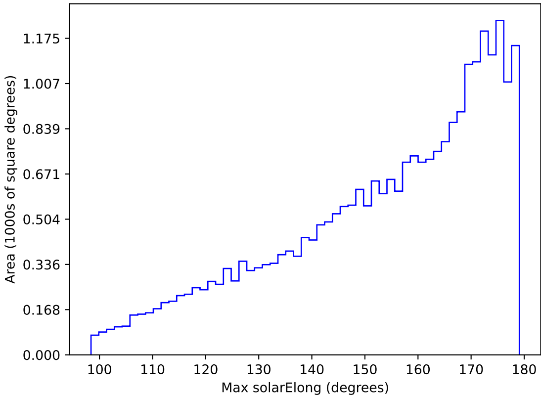
early_u_fpextra3.0_v3.4_10yrs All sky g band: Max solarElong
