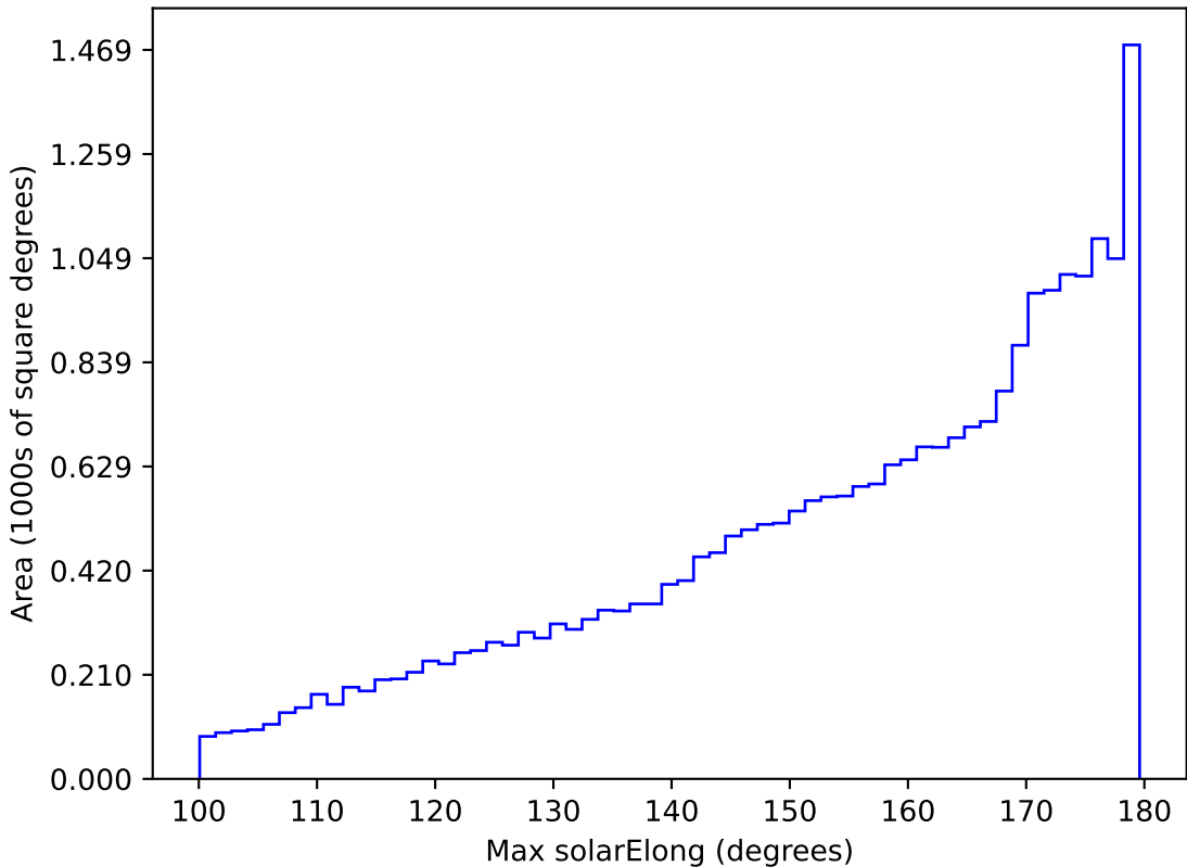
early_u_fpextra3.0_v3.4_10yrs All sky all bands: Max solarElong
