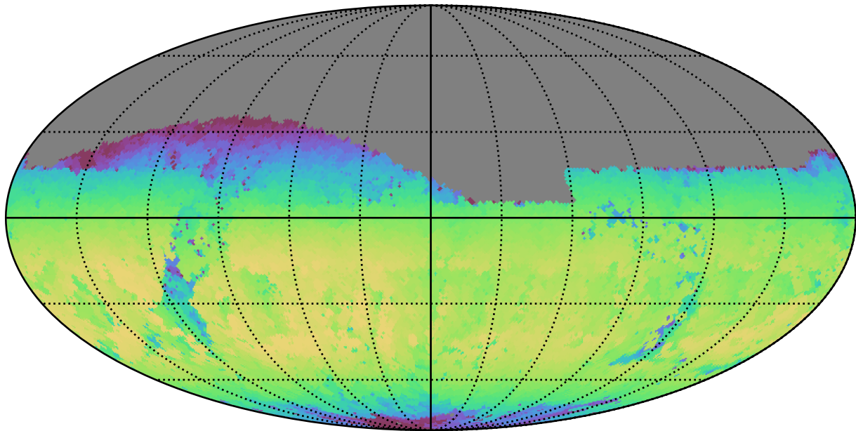
early_u_fpextra3.0_v3.4_10yrs Yr 1 z band: Max skyBrightness
