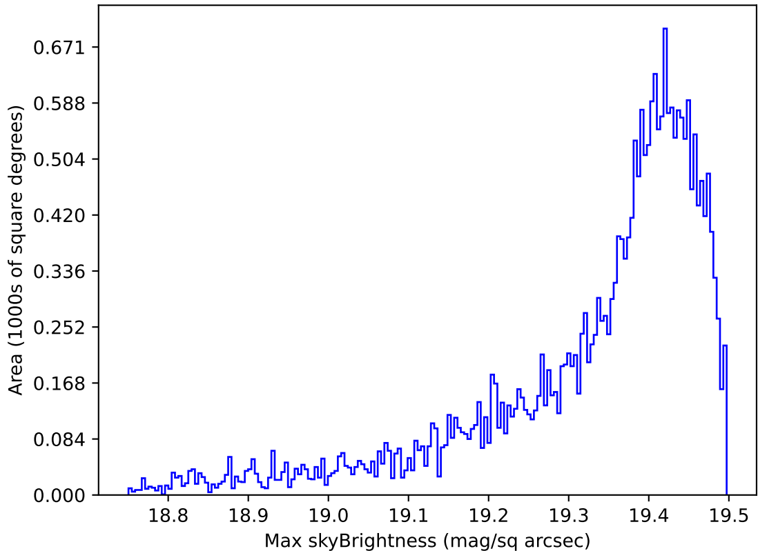
early_u_fpextra3.0_v3.4_10yrs Yr 1 z band: Max skyBrightness
