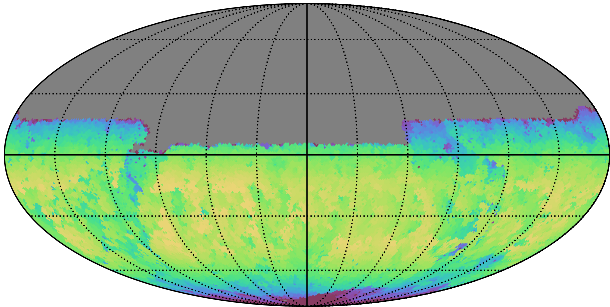
early_u_fpextra3.0_v3.4_10yrs Yr 1 y band: Max skyBrightness
