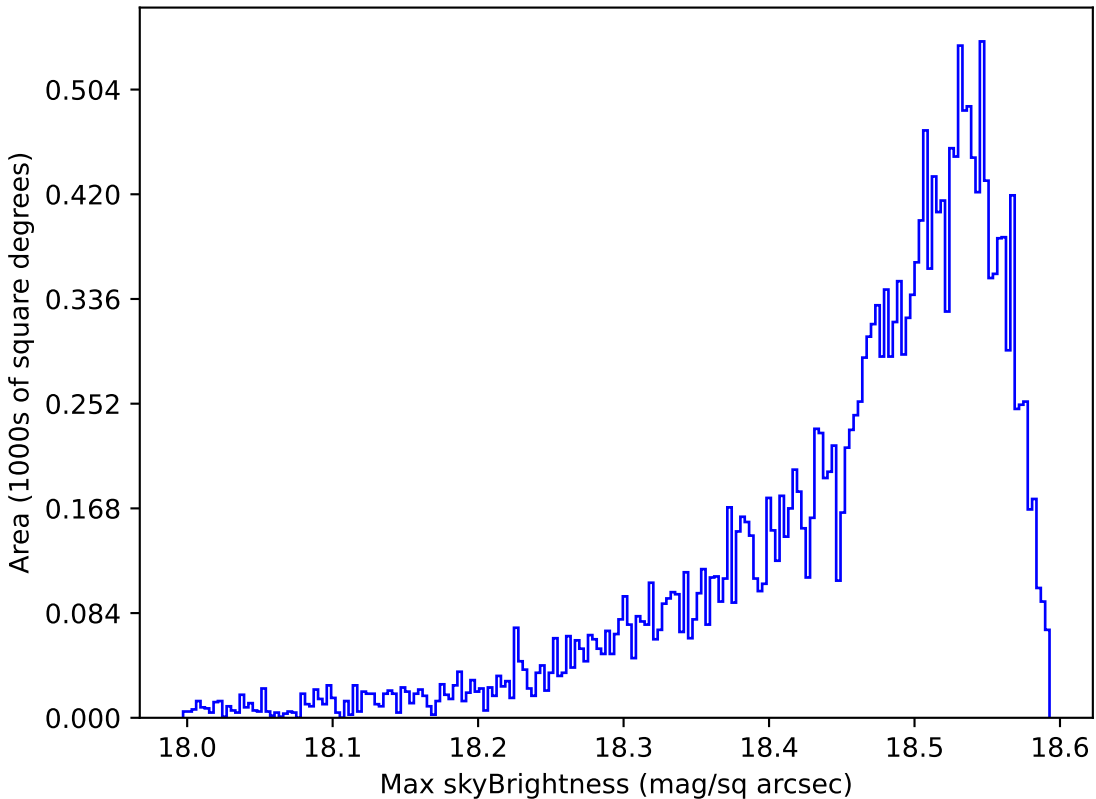
early_u_fpextra3.0_v3.4_10yrs Yr 1 y band: Max skyBrightness
