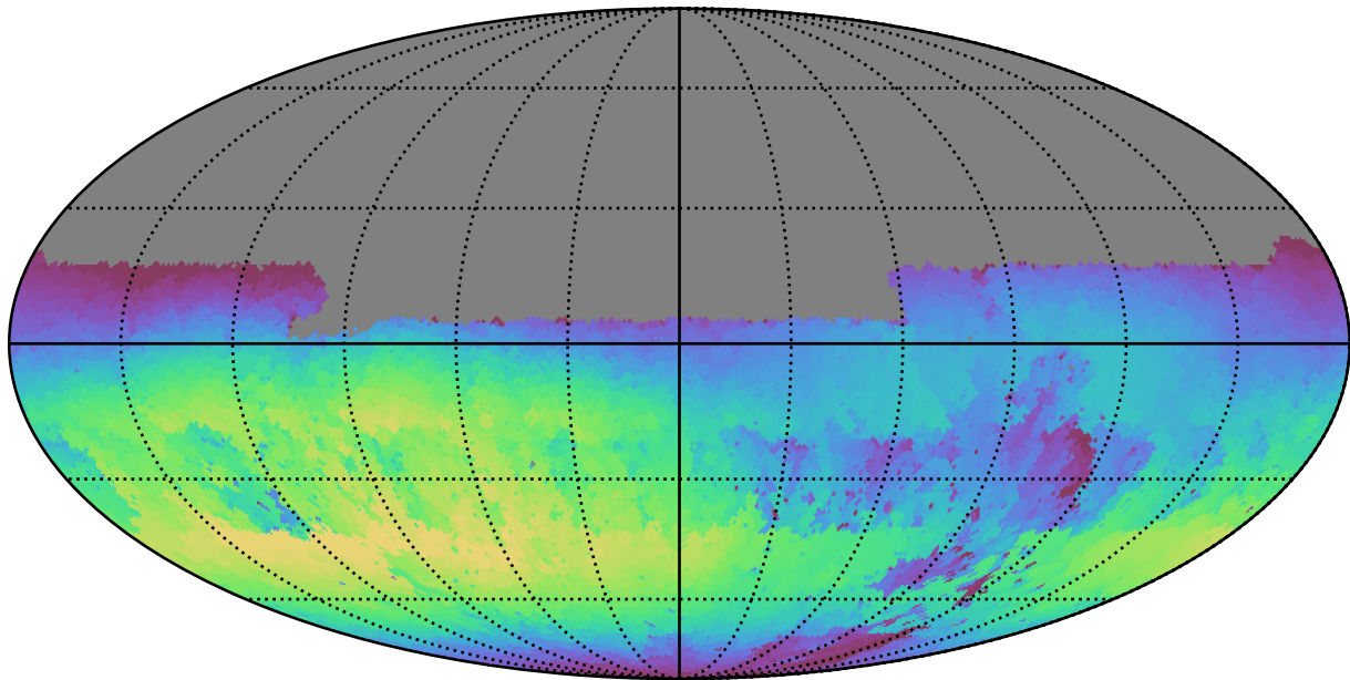
early_u_fpextra3.0_v3.4_10yrs Yr 1 u band: Max skyBrightness
