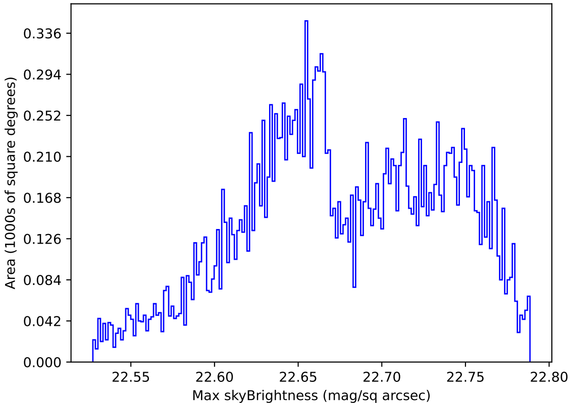
early_u_fpextra3.0_v3.4_10yrs Yr 1 u band: Max skyBrightness
