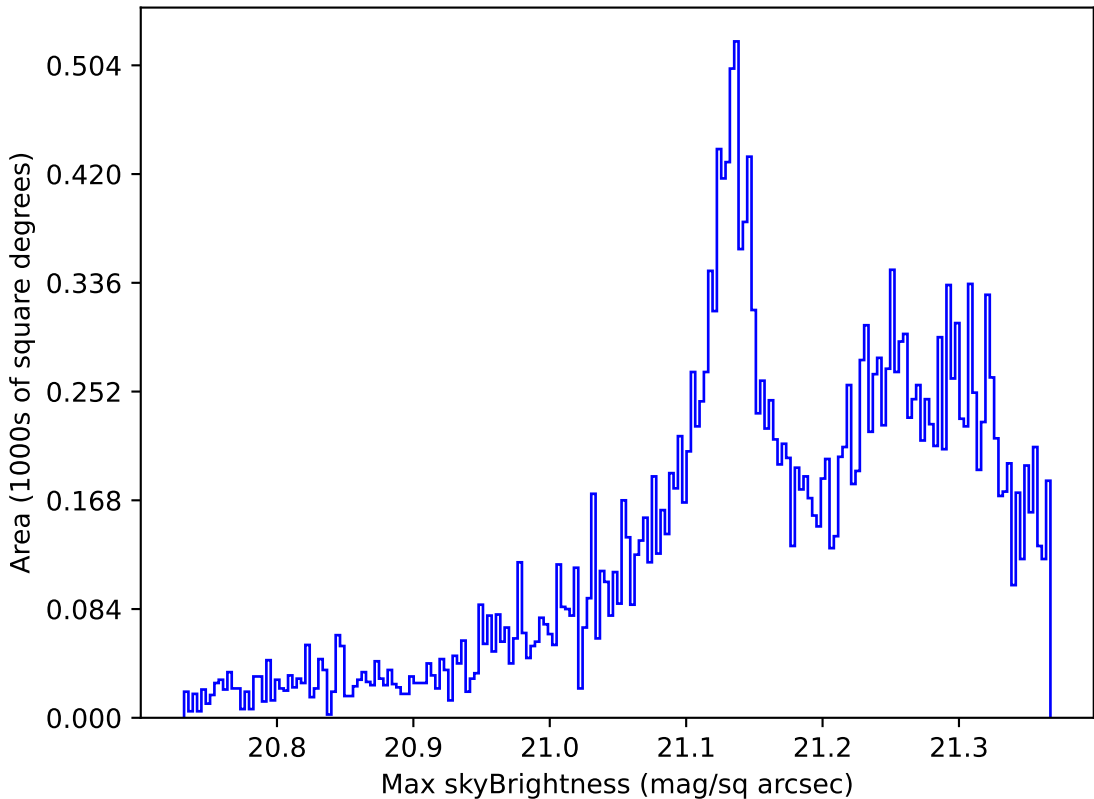
early_u_fpextra3.0_v3.4_10yrs Yr 1 r band: Max skyBrightness
