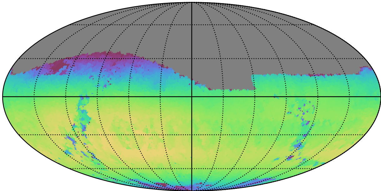
early_u_fpextra3.0_v3.4_10yrs Yr 1 i band: Max skyBrightness
