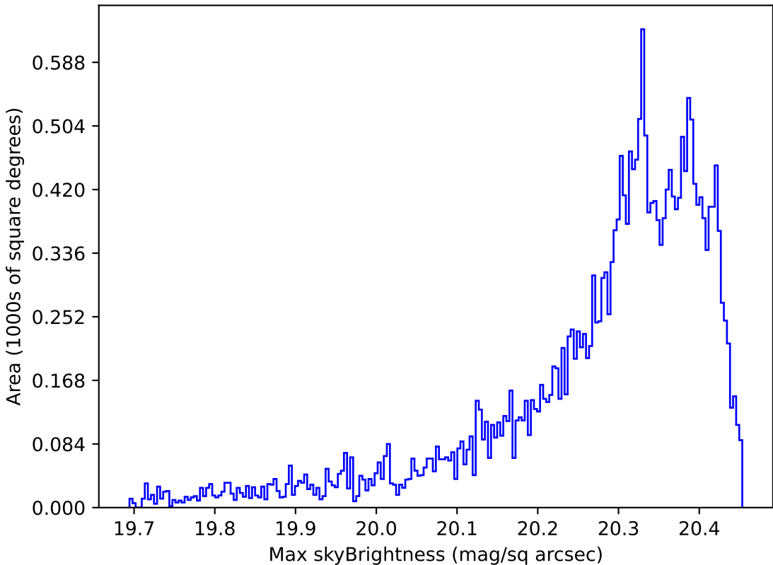
early_u_fpextra3.0_v3.4_10yrs Yr 1 i band: Max skyBrightness
