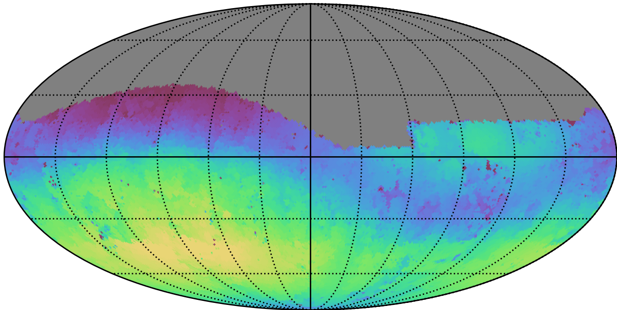
early_u_fpextra3.0_v3.4_10yrs Yr 1 g band: Max skyBrightness
