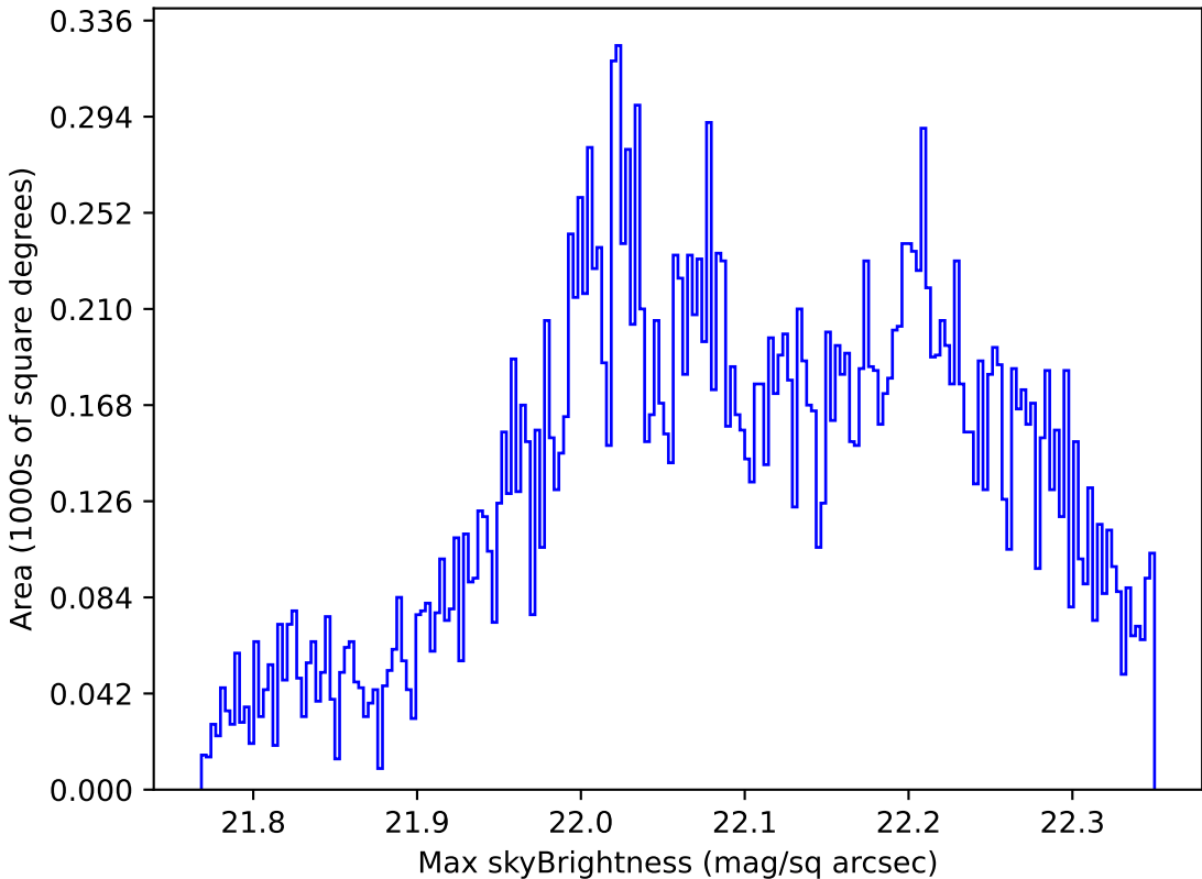
early_u_fpxextra3.0_v3.4_10yrs Yr 1 g band: Max skyBrightness
