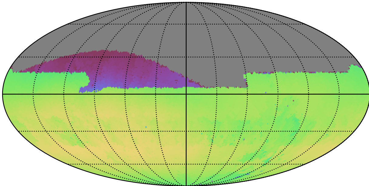
early_u_fpextra3.0_v3.4_10yrs Yr 1 all bands: Max skyBrightness
