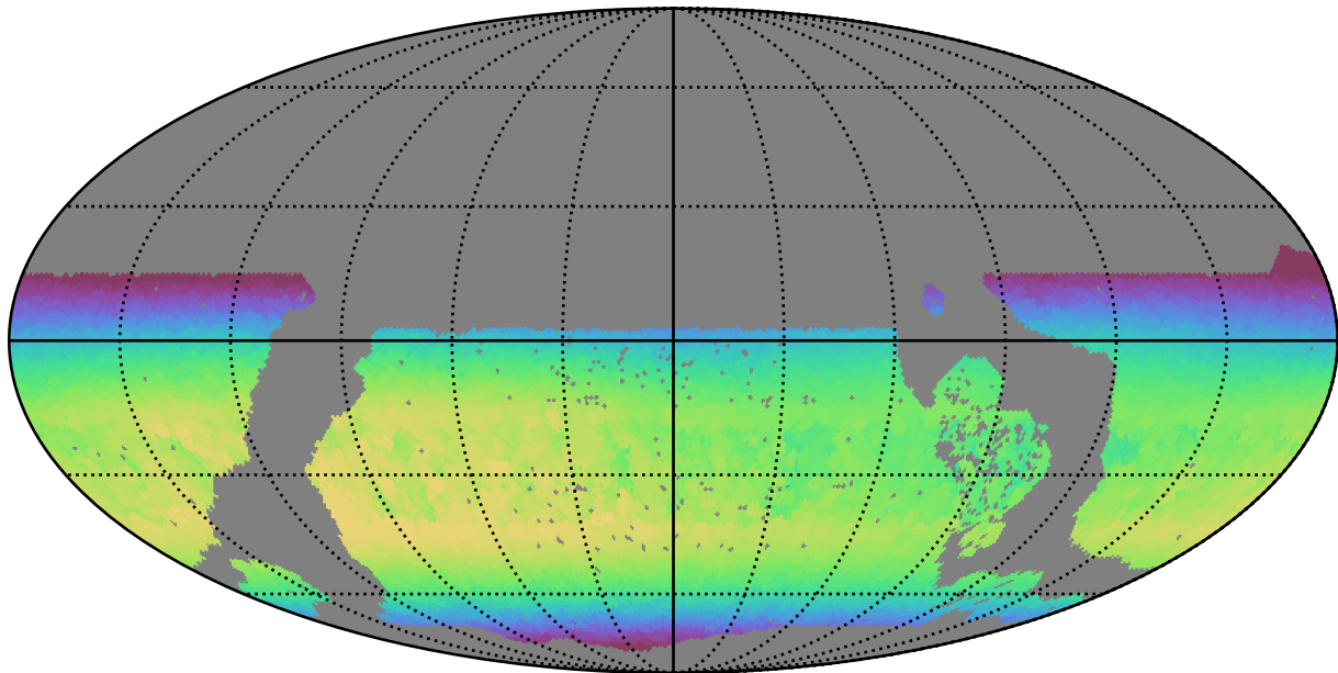
early_u_fpextra3.0_v3.4_10yrs WFD z band: Max skyBrightness
