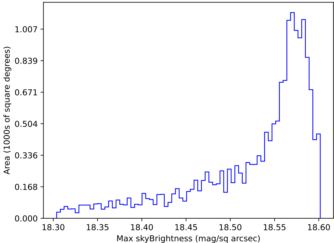
early_u_fpextra3.0_v3.4_10yrs WFD y band: Max skyBrightness
