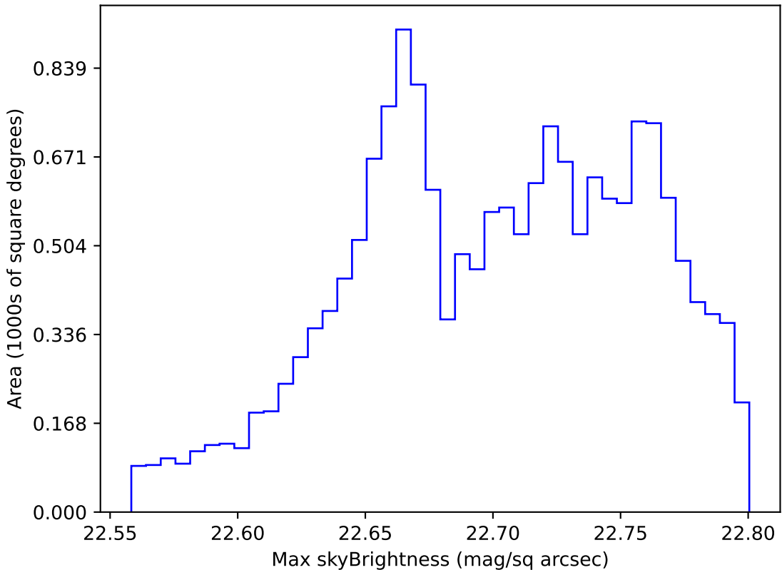
early_u_fpextra3.0_v3.4_10yrs WFD u band: Max skyBrightness
