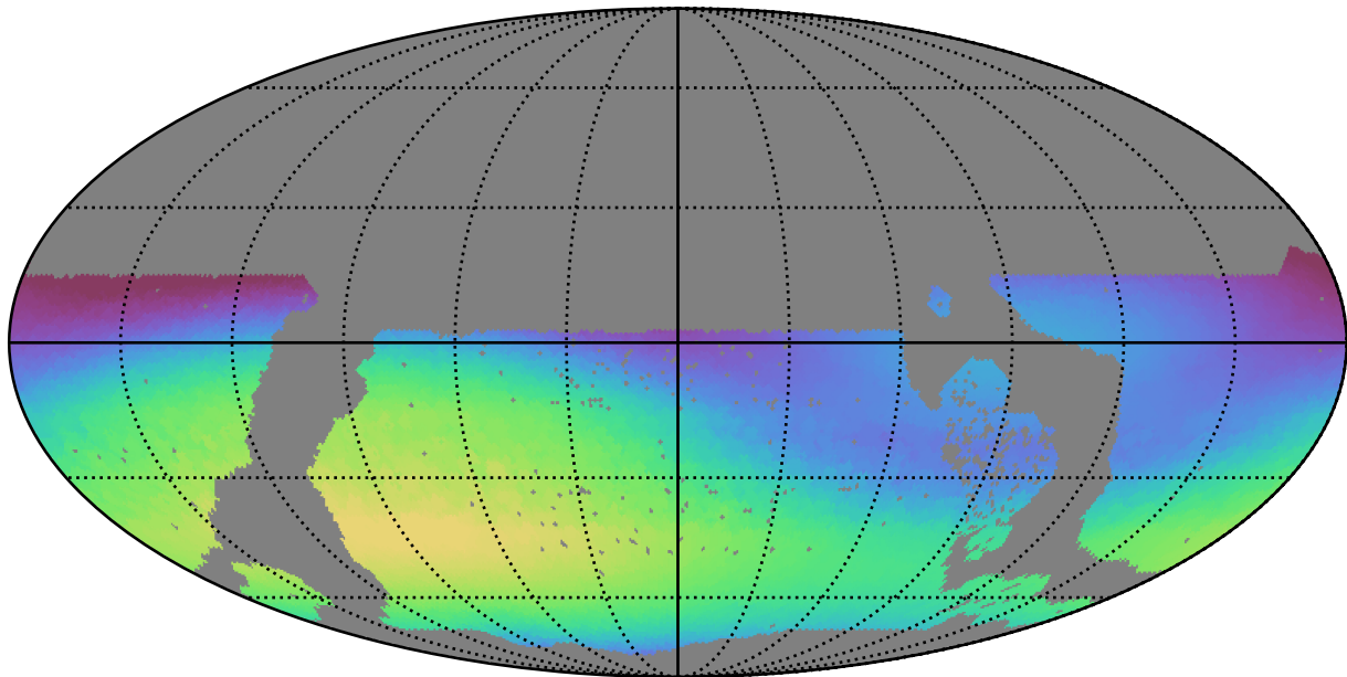
early_u_fpextra3.0_v3.4_10yrs WFD r band: Max skyBrightness
