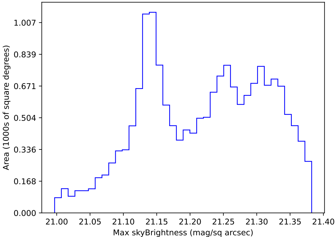
early_u_fpextra3.0_v3.4_10yrs WFD r band: Max skyBrightness
