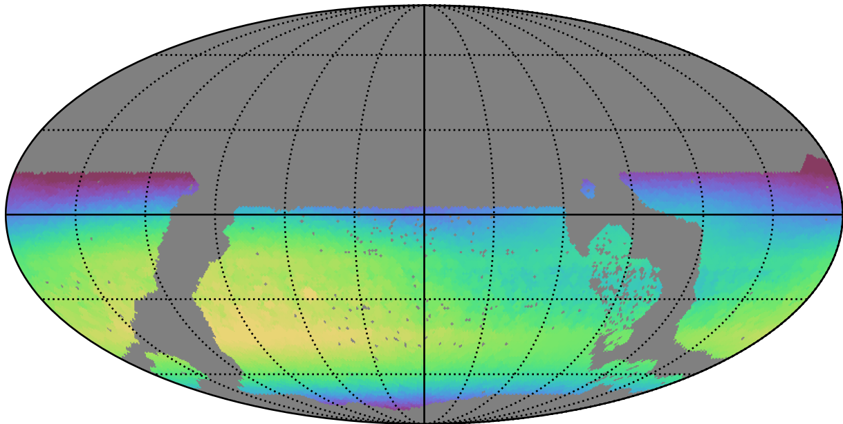
early_u_fpextra3.0_v3.4_10yrs WFD i band: Max skyBrightness
