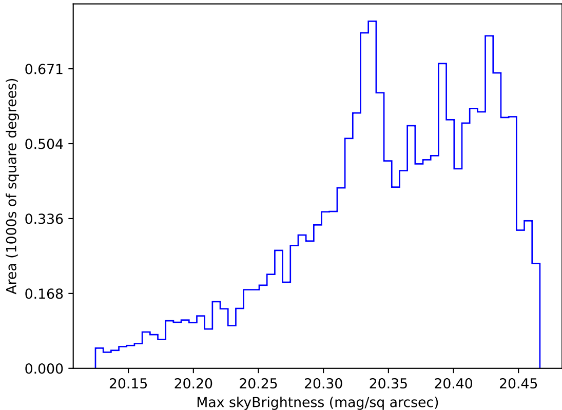
early_u_fpextra3.0_v3.4_10yrs WFD i band: Max skyBrightness
