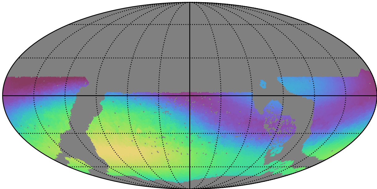
early_u_fpextra3.0_v3.4_10yrs WFD g band: Max skyBrightness
