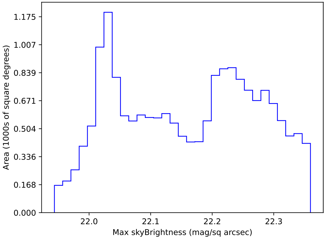
early_u_fpextra3.0_v3.4_10yrs WFD g band: Max skyBrightness
