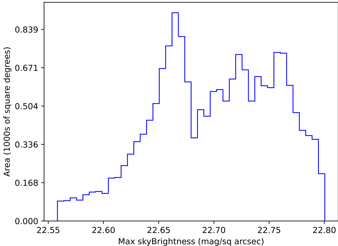
early_u_fpextra3.0_v3.4_10yrs WFD all bands: Max skyBrightness
