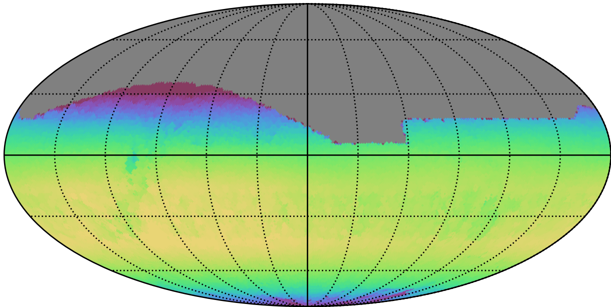
early_u_fpextra3.0_v3.4_10yrs All sky z band: Max skyBrightness
