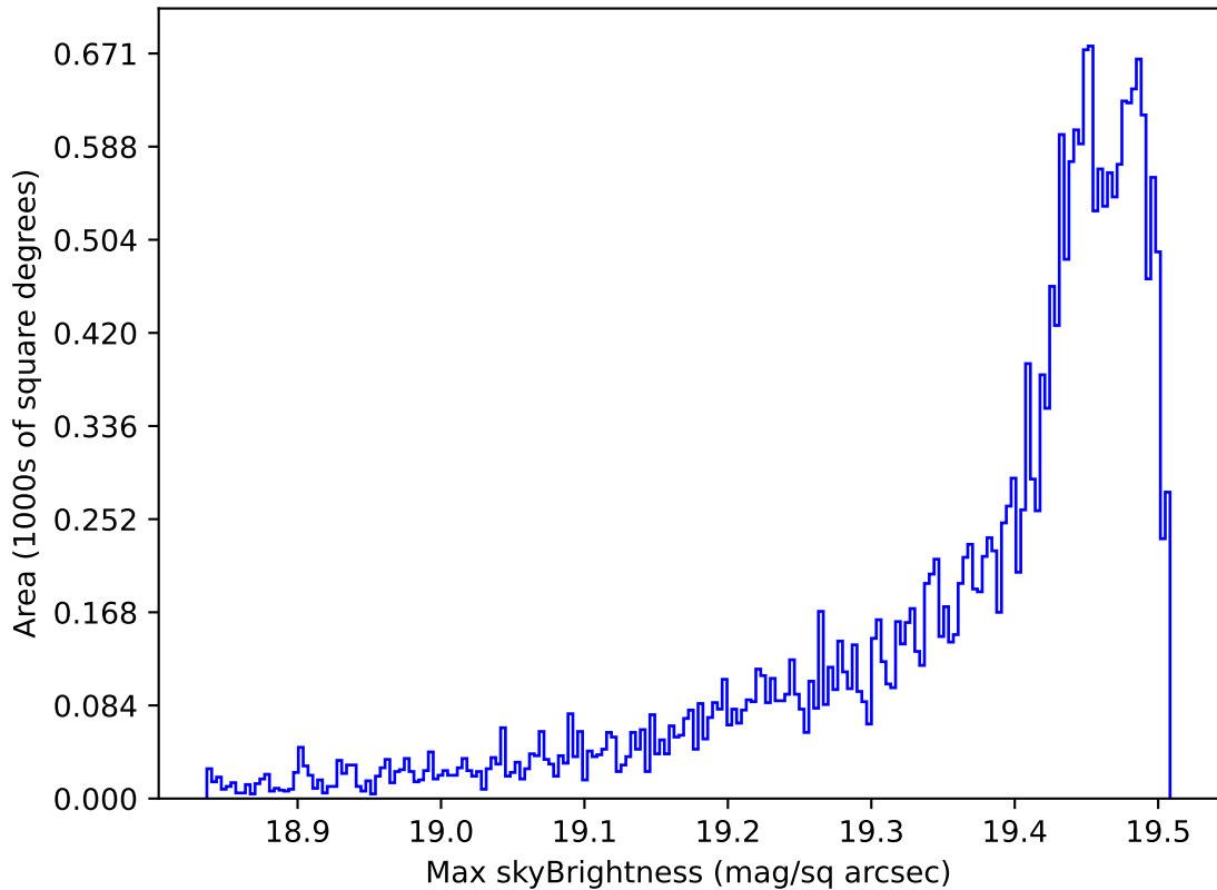
early_u_fpextra3.0_v3.4_10yrs All sky z band: Max skyBrightness
