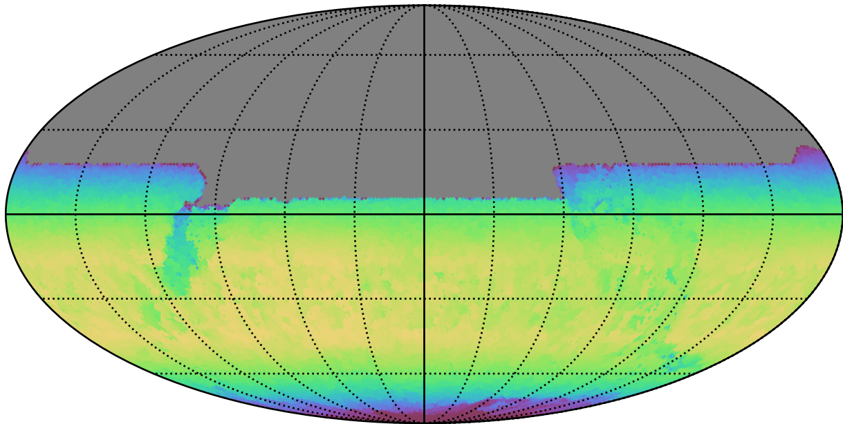
early_u_fpextra3.0_v3.4_10yrs All sky y band: Max skyBrightness
