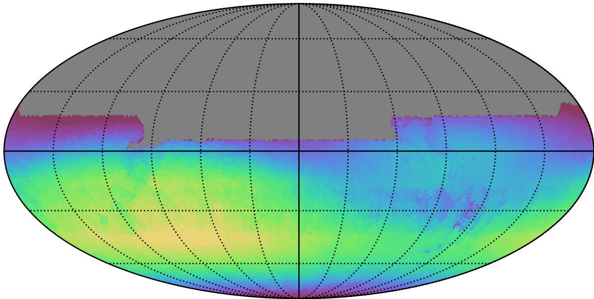
early_u_fpextra3.0_v3.4_10yrs All sky u band: Max skyBrightness
