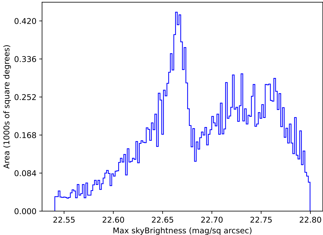
early_u_fpextra3.0_v3.4_10yrs All sky u band: Max skyBrightness
