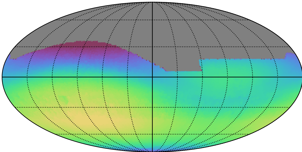
early_u_fpextra3.0_v3.4_10yrs All sky r band: Max skyBrightness
