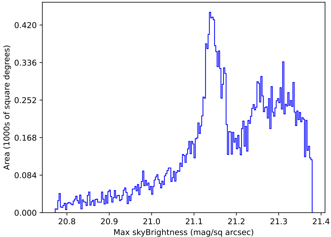
early_u_fpextra3.0_v3.4_10yrs All sky r band: Max skyBrightness
