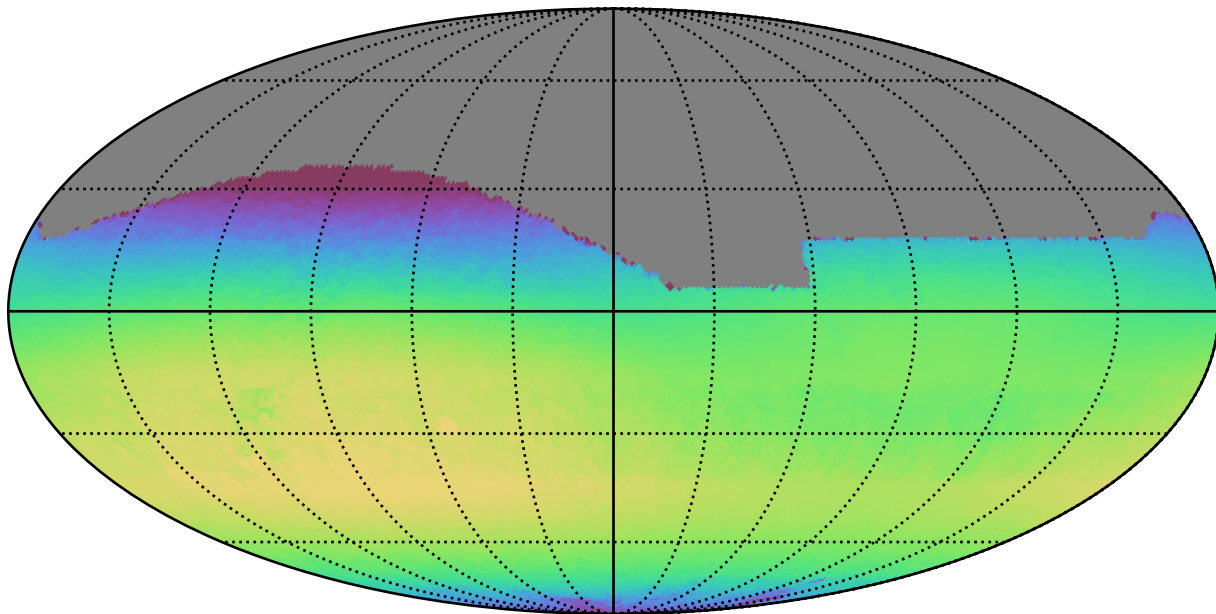
early_u_fpextra3.0_v3.4_10yrs All sky i band: Max skyBrightness
