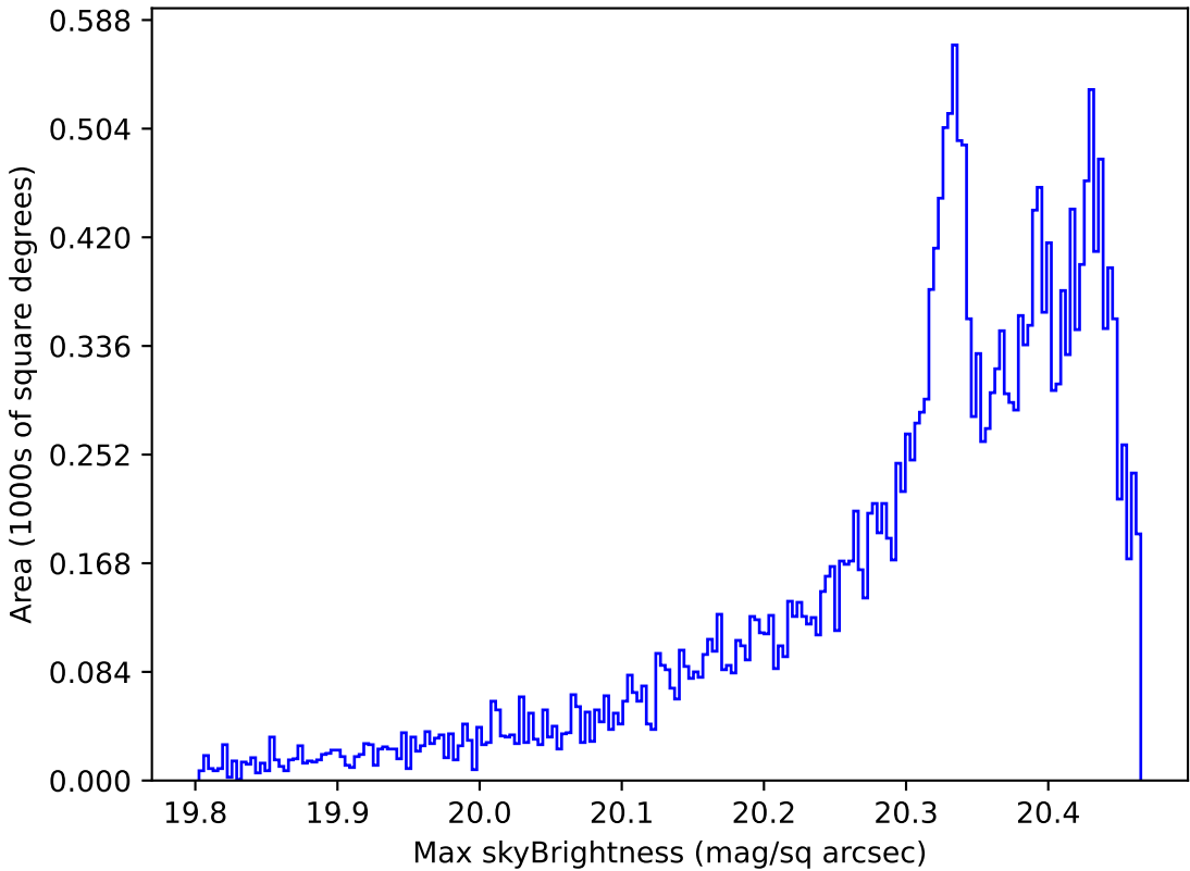
early_u_fpextra3.0_v3.4_10yrs All sky i band: Max skyBrightness
