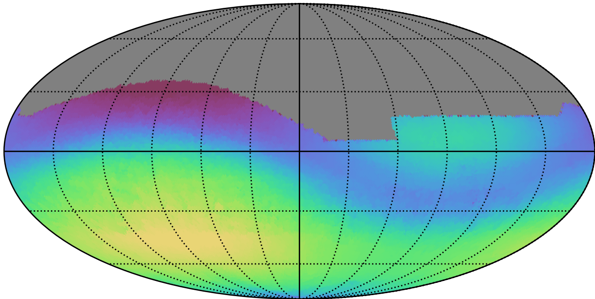
early_u_fpextra3.0_v3.4_10yrs All sky g band: Max skyBrightness
