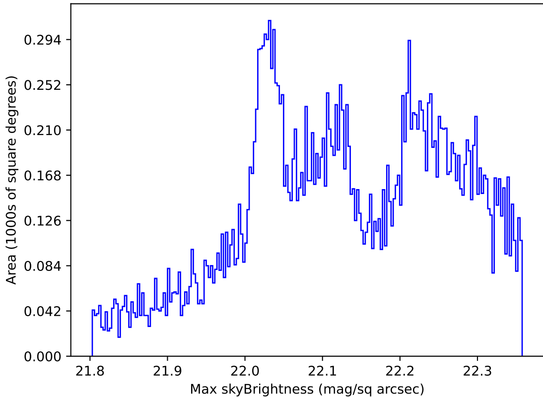
early_u_fpextra3.0_v3.4_10yrs All sky g band: Max skyBrightness
