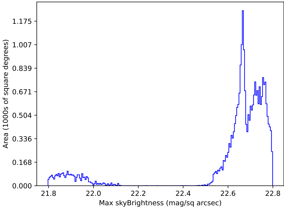
early_u_fpextra3.0_v3.4_10yrs All sky all bands: Max skyBrightness
