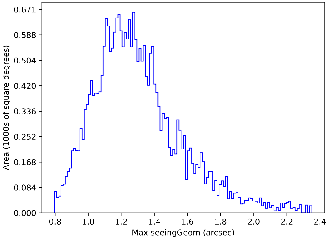
early_u_fpextra3.0_v3.4_10yrs Yr 1 z band: Max seeingGeom
