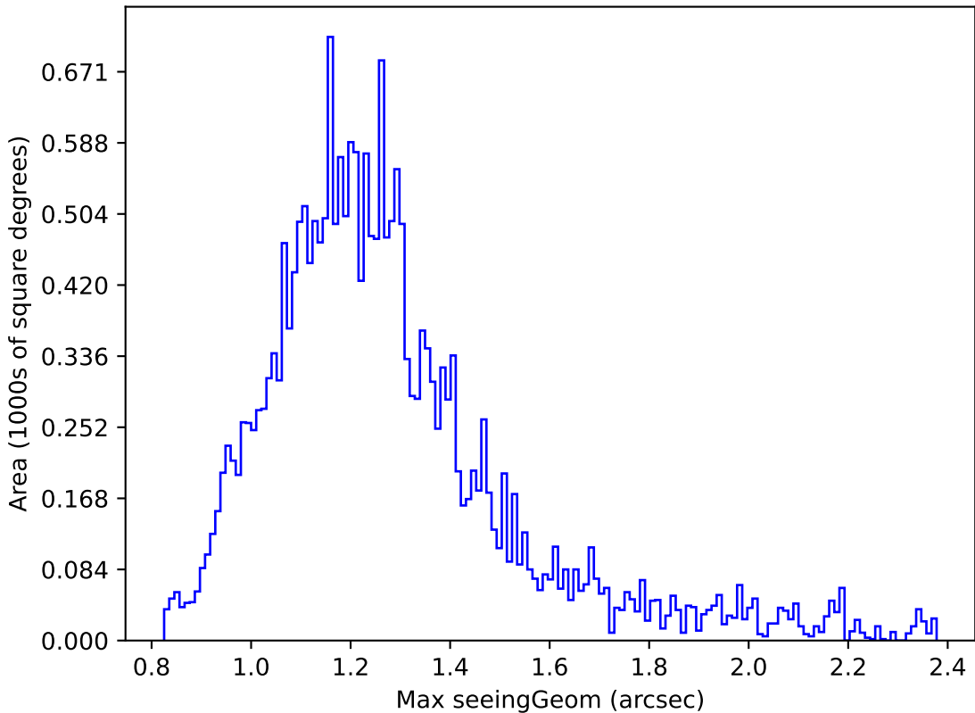
early_u_fpextra3.0_v3.4_10yrs Yr 1 y band: Max seeingGeom
