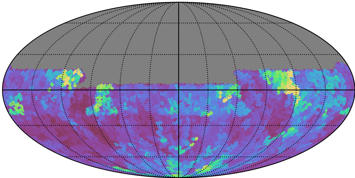
early_u_fpextra3.0_v3.4_10yrs Yr 1 u band: Max seeingGeom
