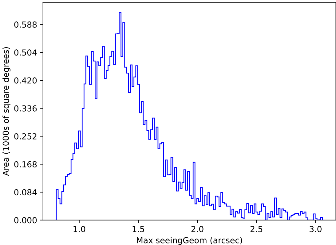
early_u_fpextra3.0_v3.4_10yrs Yr 1 u band: Max seeingGeom
