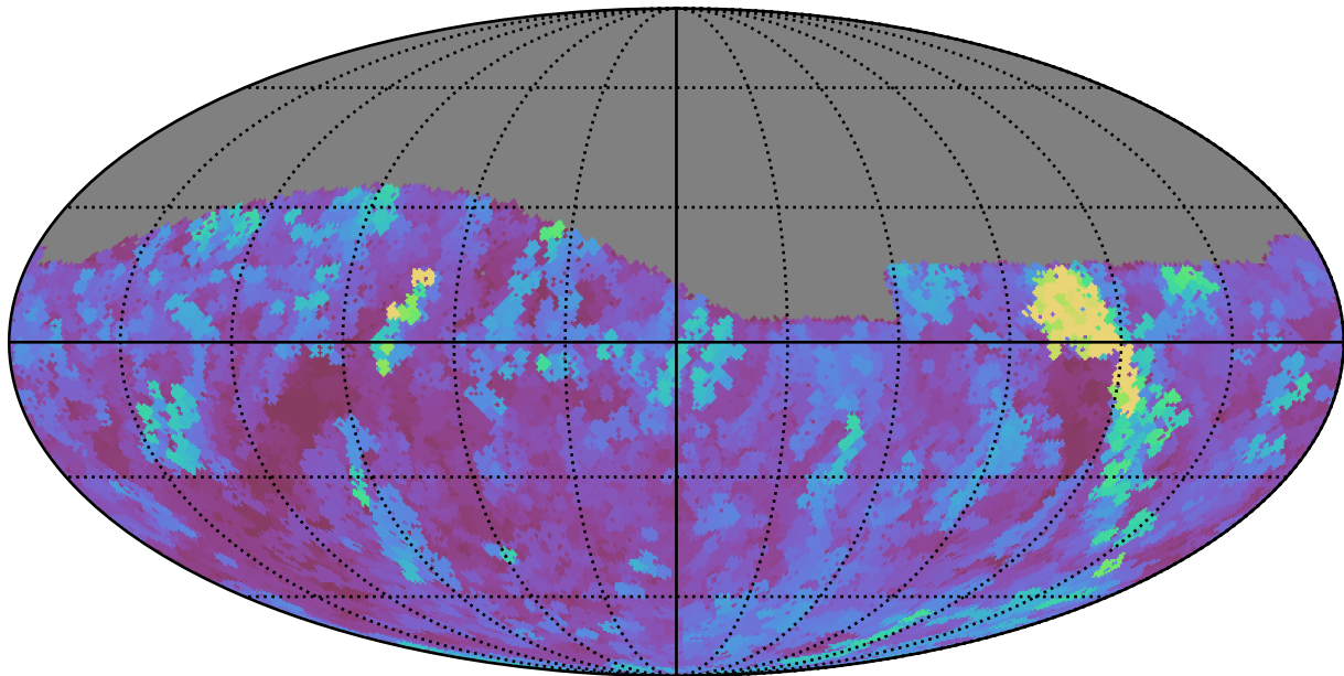
early_u_fpextra3.0_v3.4_10yrs Yr 1 r band: Max seeingGeom
