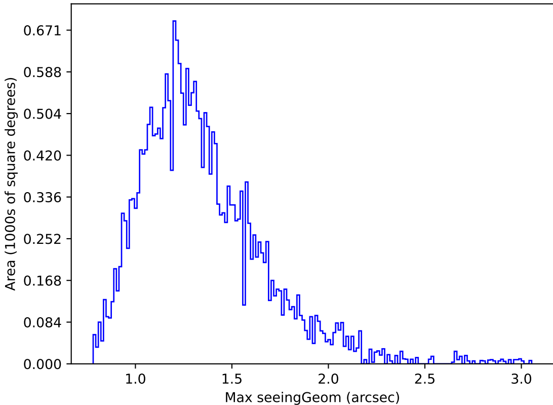
early_u_fpextra3.0_v3.4_10yrs Yr 1 r band: Max seeingGeom
