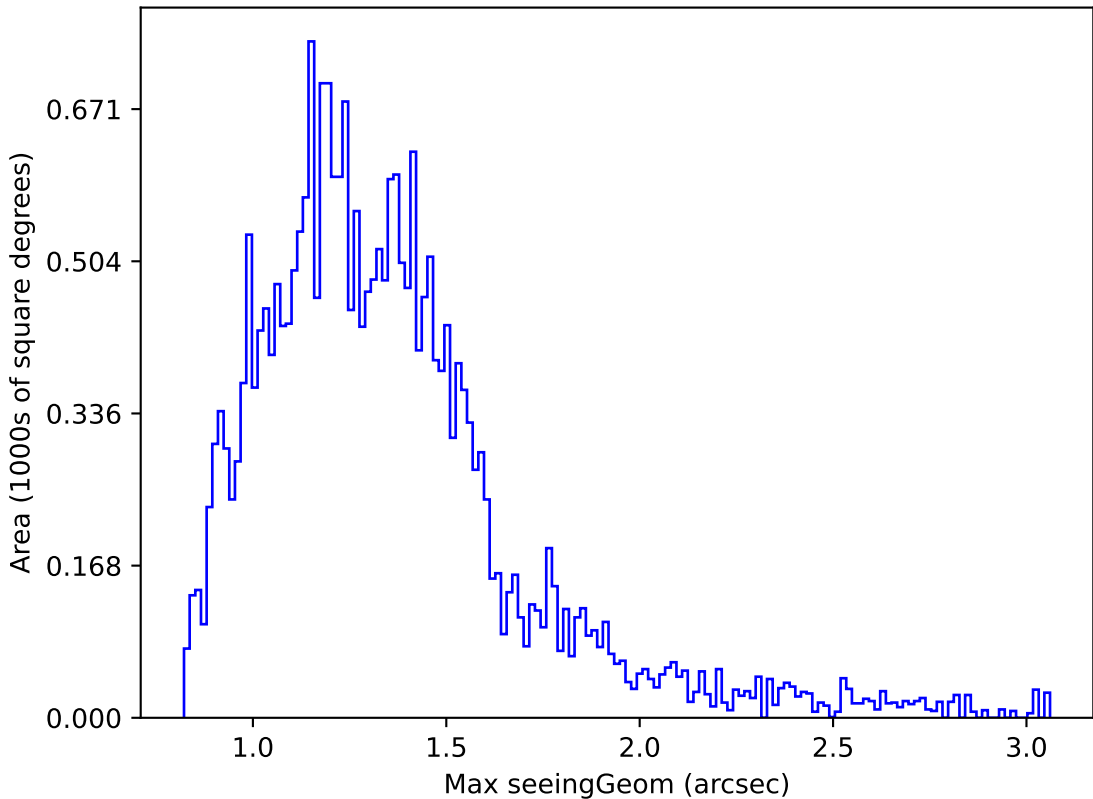
early_u_fpextra3.0_v3.4_10yrs Yr 1 i band: Max seeingGeom
