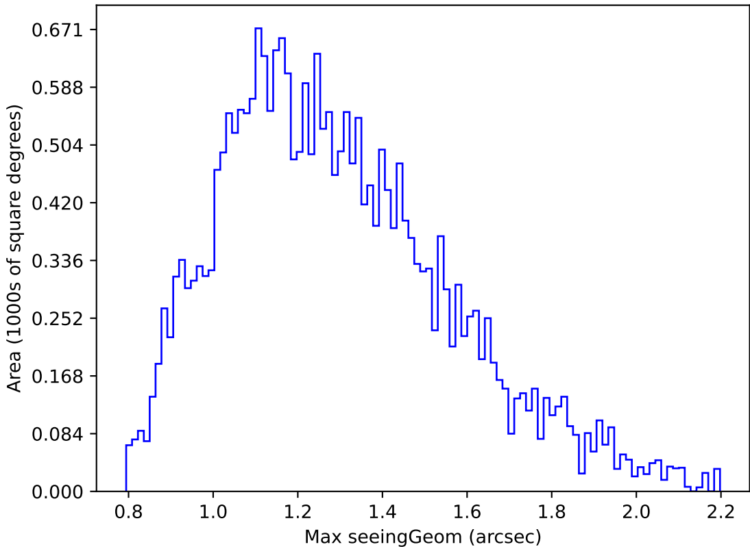
early_u_fpextra3.0_v3.4_10yrs Yr 1 g band: Max seeingGeom
